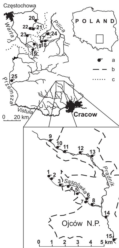
Fig. 1. Location of the area (the Krakow-Częstochowa Upland) and springs under investigation: no. 1–15 – southern group of springs situated along the Sąpówka stream and the Prądnik stream, no. 16–25 – northern group of springs situated in the catchments of the Pilica River, Warta River and Przemsza River; alkaline springs no. 19 and 25, a – springs, b – borders of the Ojców National Park, c – watershed between the Vistula and Oder drainage basins, after Galas (2005).
